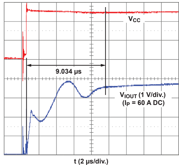
Power-on Delay
