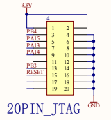
20PIN_JTAG
